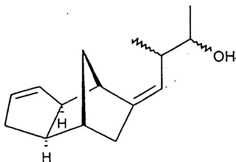
rac- 3
