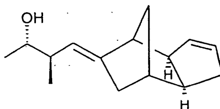
ent-B
