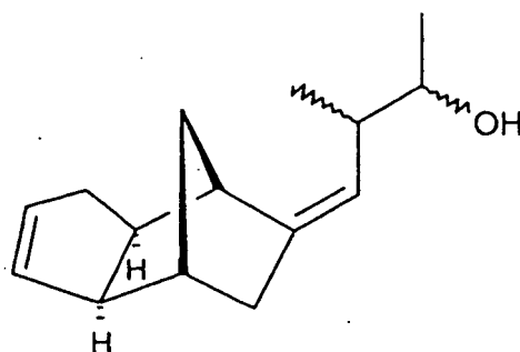
rac- 4
