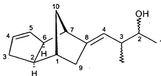
rac-1
