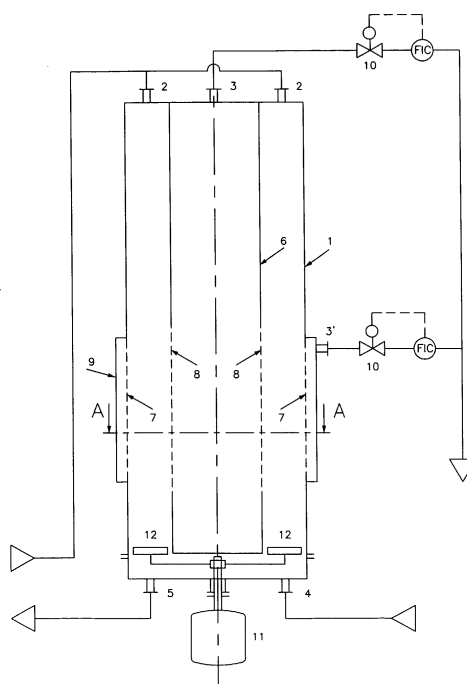
figure:1 hydraulic annular washcolumn
