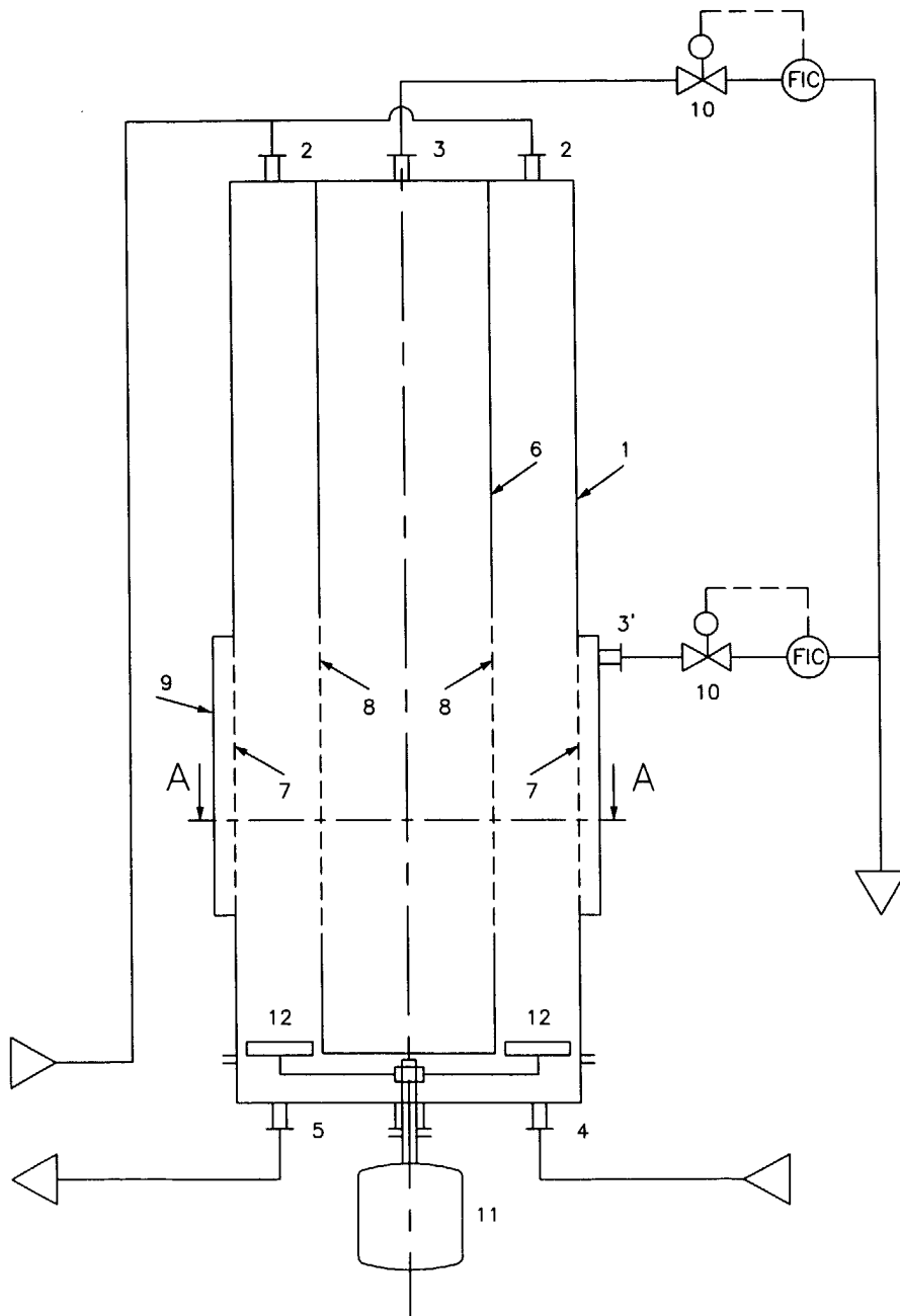
figure:1 hydraulic annular washcolumn
