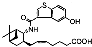
PGD 2 Receptor antagonist (B-2)
