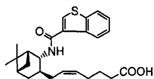
PGD 2 Receptor antagonist (B-1)
