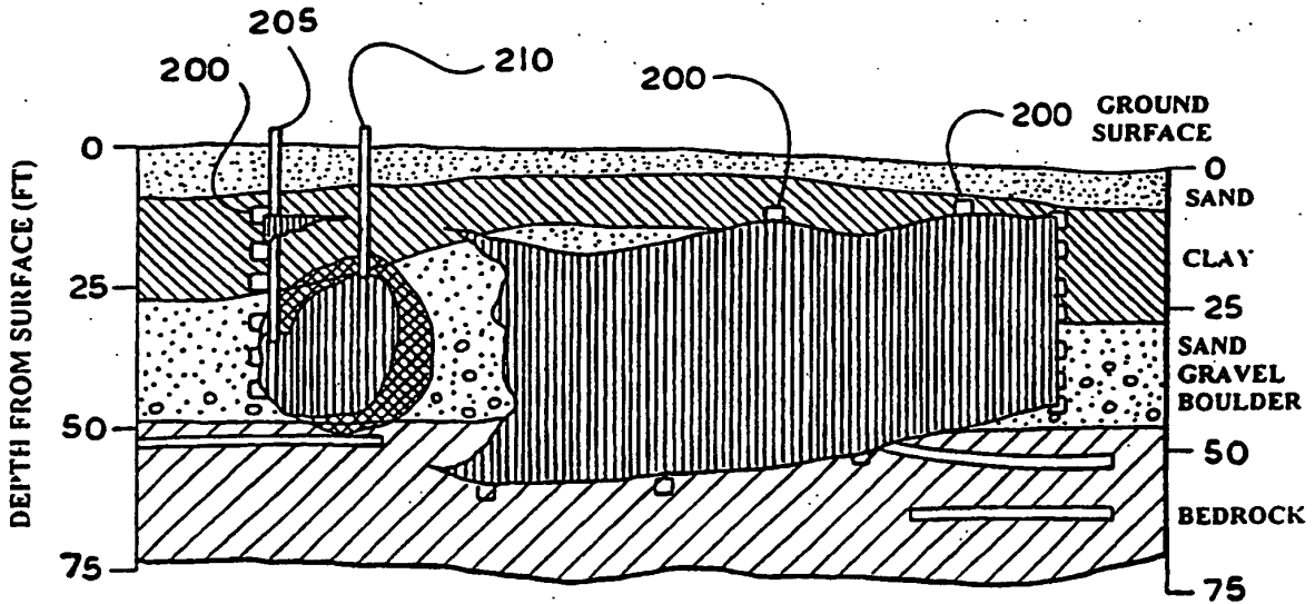
INDUCED VOLTAGES FROM PROPAGATING FRACTURE.
