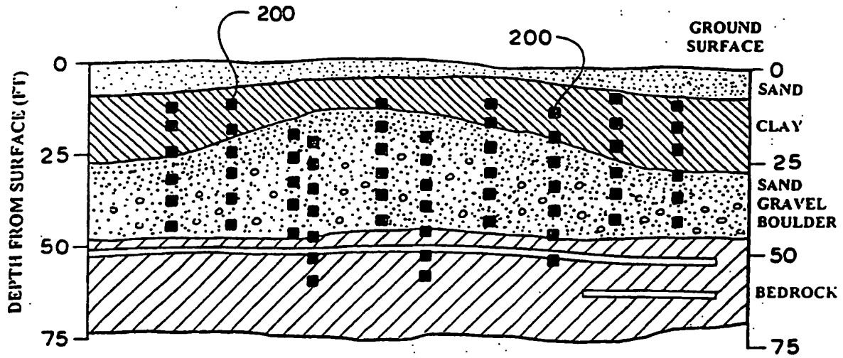
DOWN HOLE RESISTIVITY RECEIVERS.
