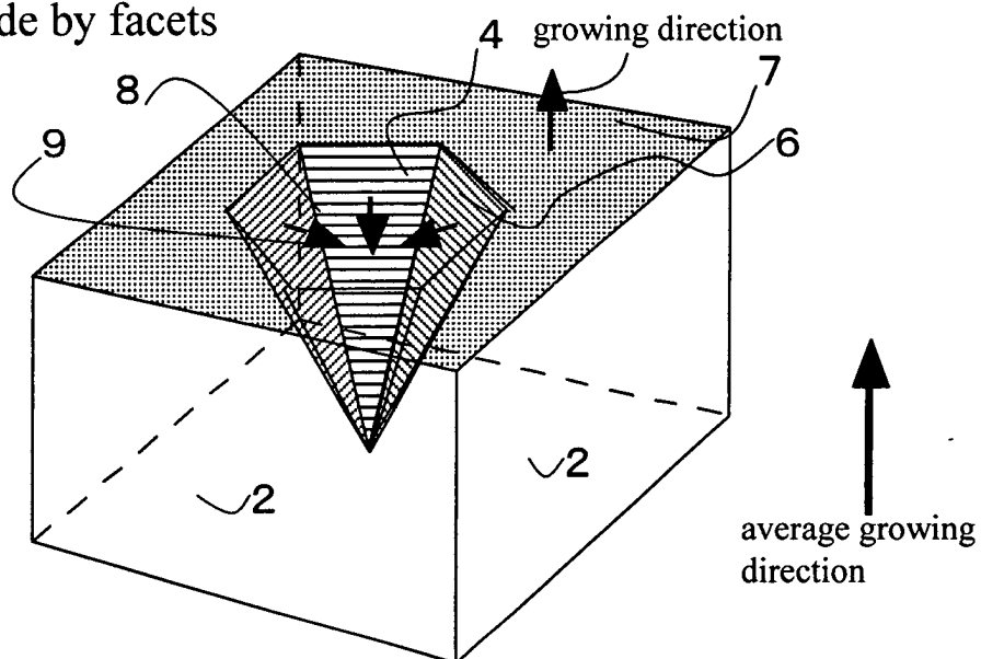
(b) after continual growth
