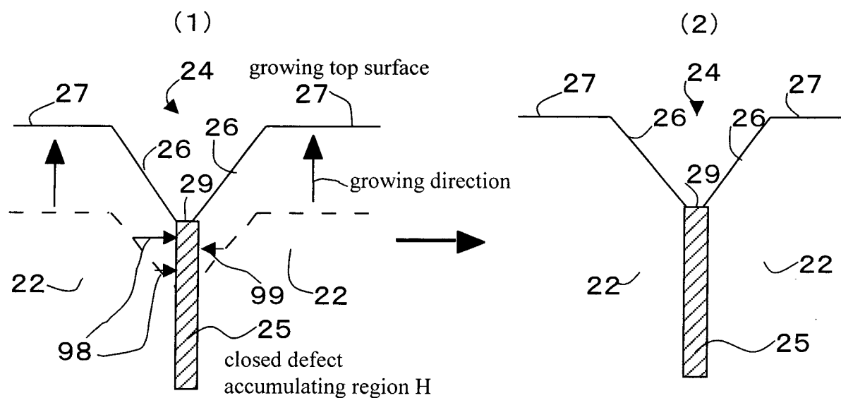
Fig.4 growing method of the present invention
