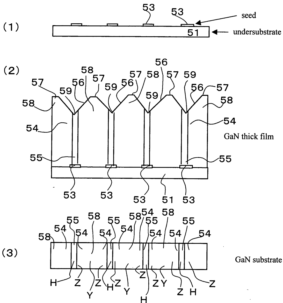
Fig.12 Embodiment 2 processes of producing a GaN substrate
