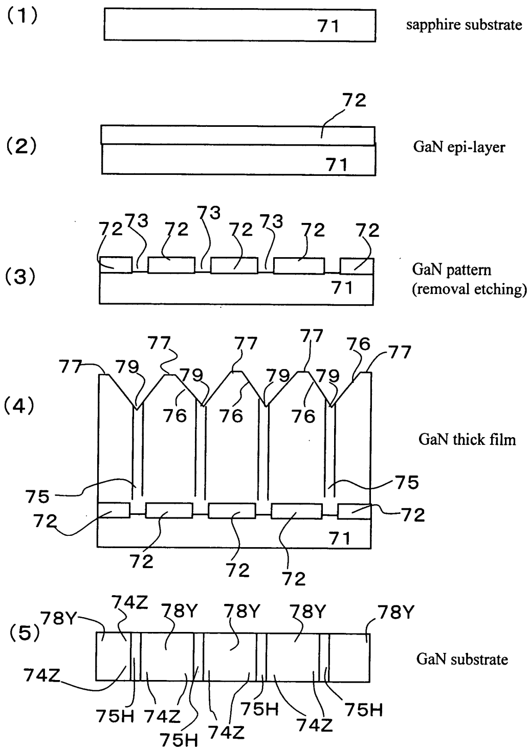
Fig.14 Processes of producing a GaN substrate
