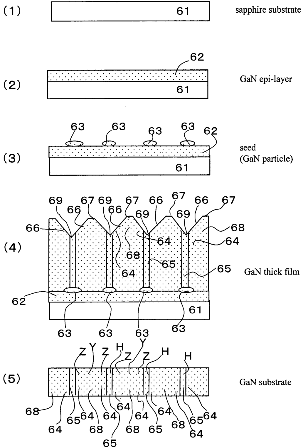
Fig.13 Embodiment 4 Processes of producing a GaN substrate
