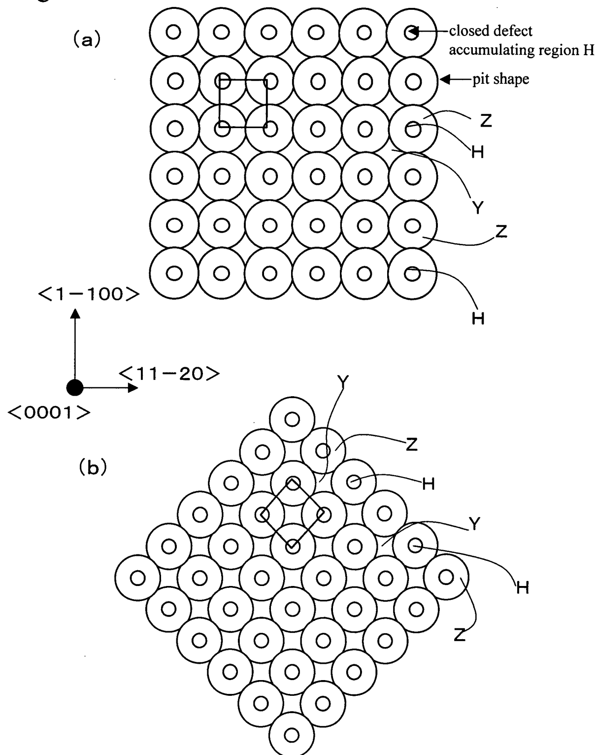
Fig.9 four-fold rotational arrangement on undersubstrate
