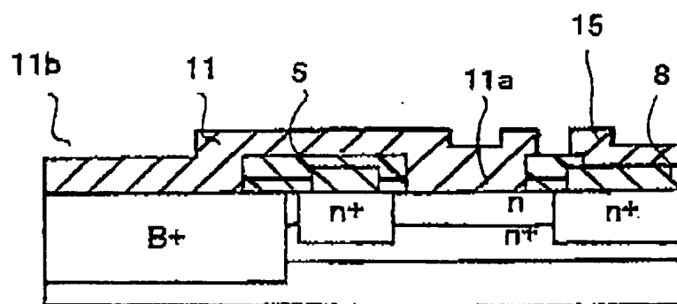
FIG.7D
