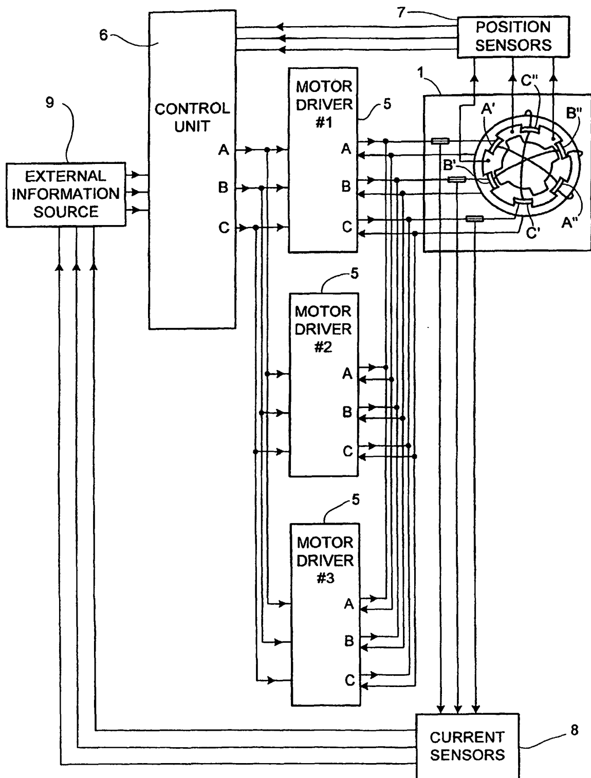
FIG. 2 PRIOR ART
