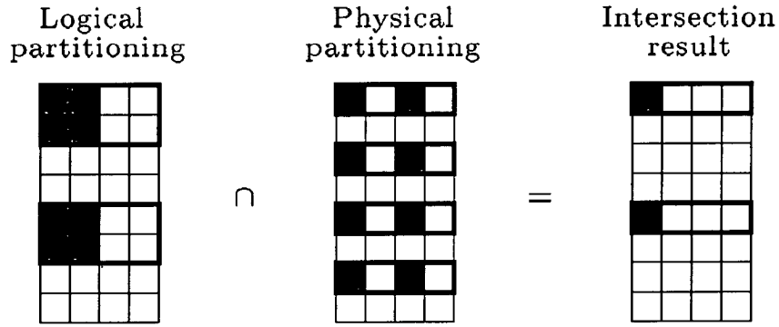
(a) Logical and physical partitioning(array form)
