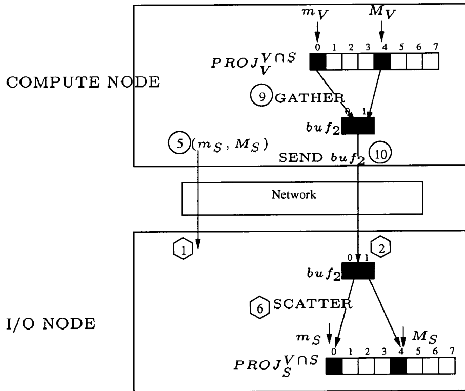
(b) Communication between compute node and I/O node
