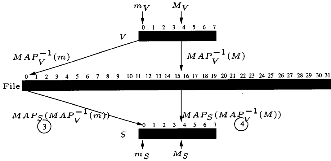
(a) Compute node maps m and M on the subfile
