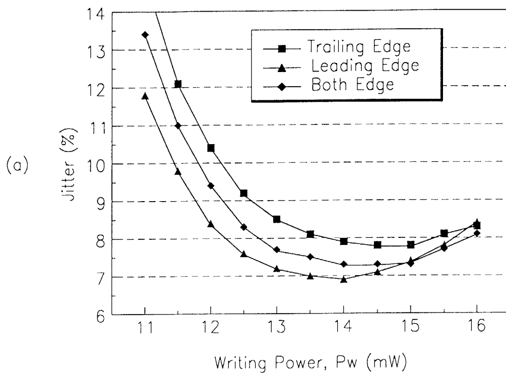
FIG. 16 (PRIOR ART)
