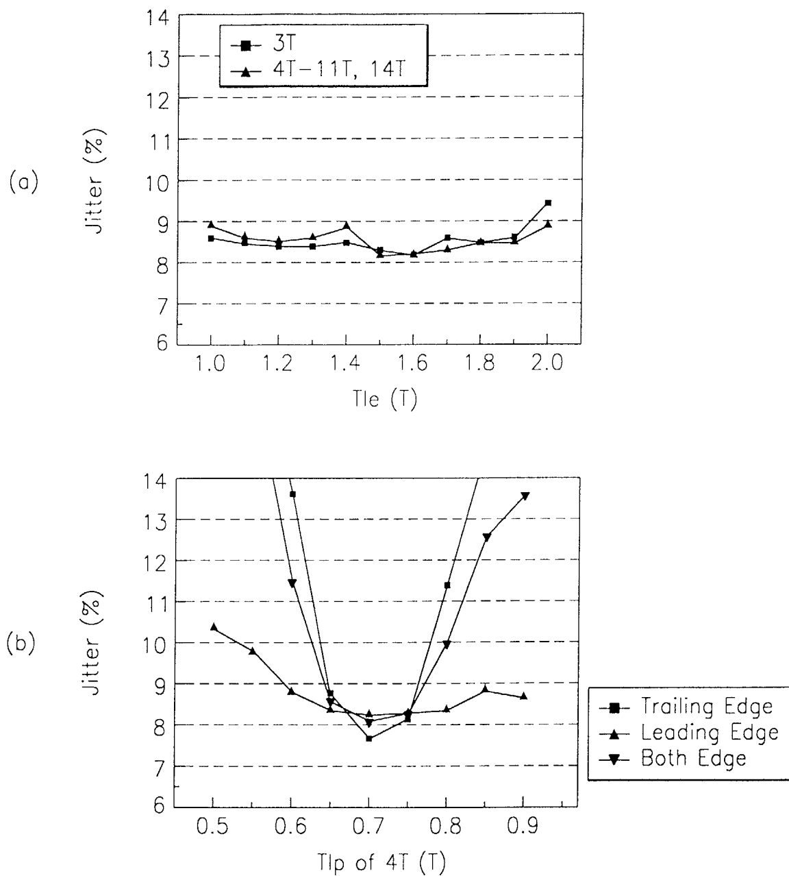
FIG. 13 (PRIOR ART)
