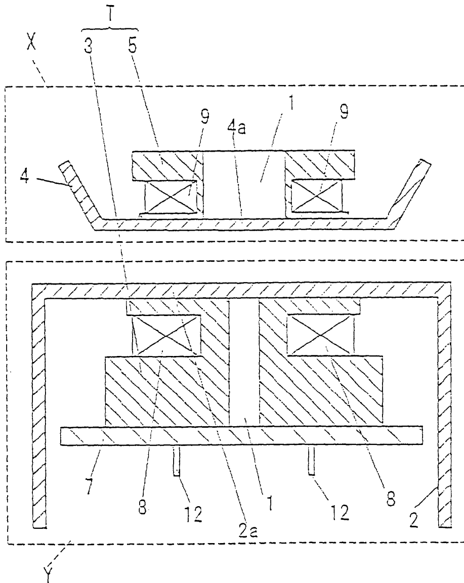
FIGURE 6 PRIOR ART
