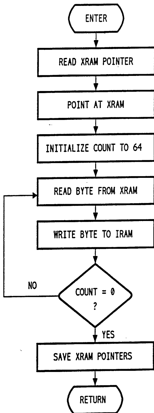
FIG 26E REPROG/READ A BLOCK
