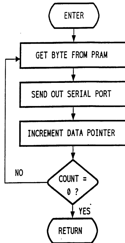
FIG 27L FIO DOWN LD/NEIGHBOR/ SEND_NEIGH/SEND_BYTE
