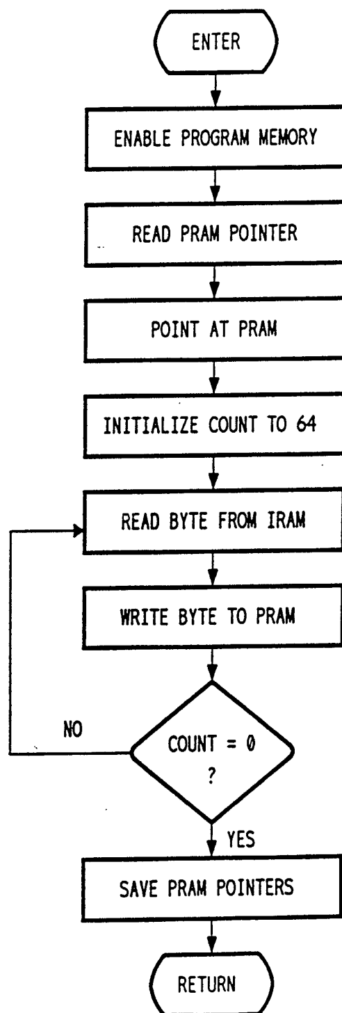
FIG 26F REPROG/WRITE A BLOCK
