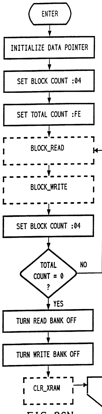
FIG 26N FIO DOWN LD/NEW PROGRAM/LJMP REPROG
