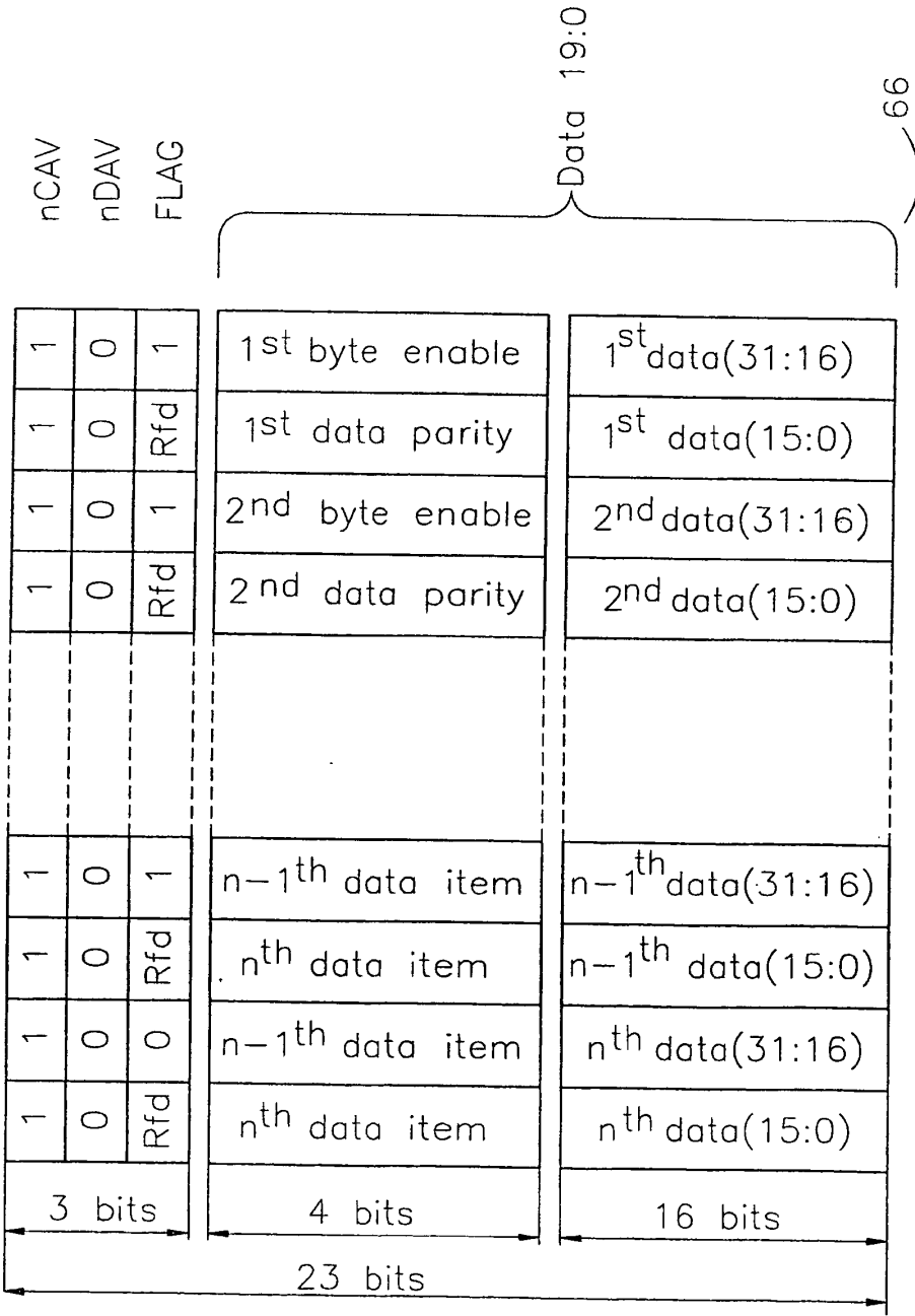
Example implementation showing i960-style burst local bus protocol carried on HP-GLINK physical layer
