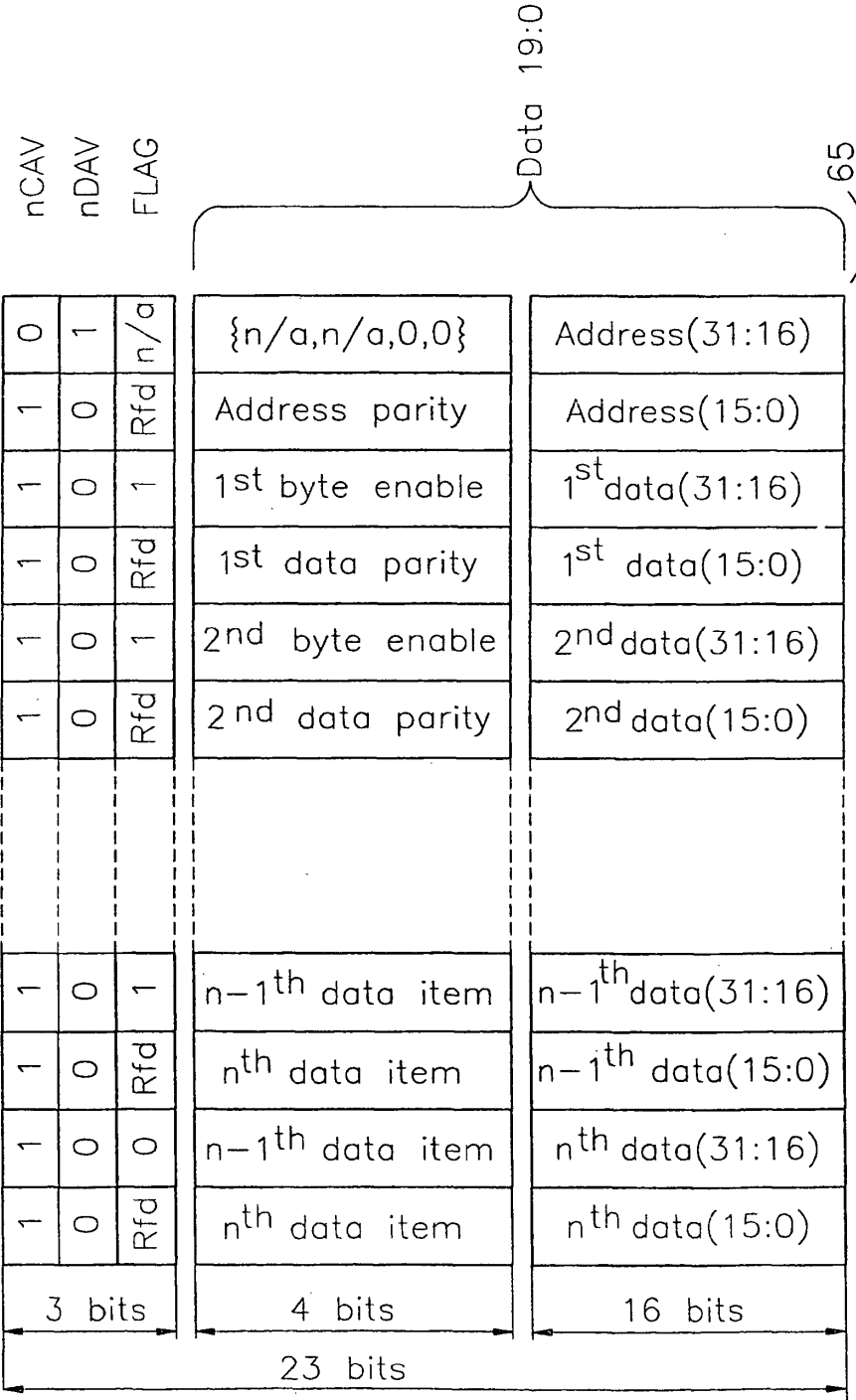
Example implementation showing i960-style burst local bus protocol carried on HP-GLINK physical layer
