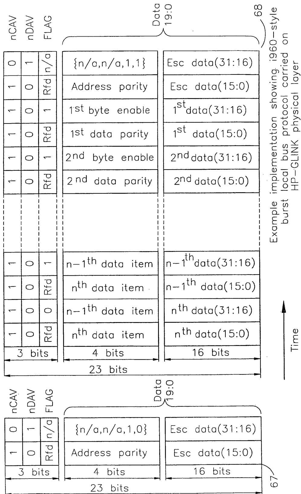
Current protocol embodiment (Escape packets without / with payloads)
