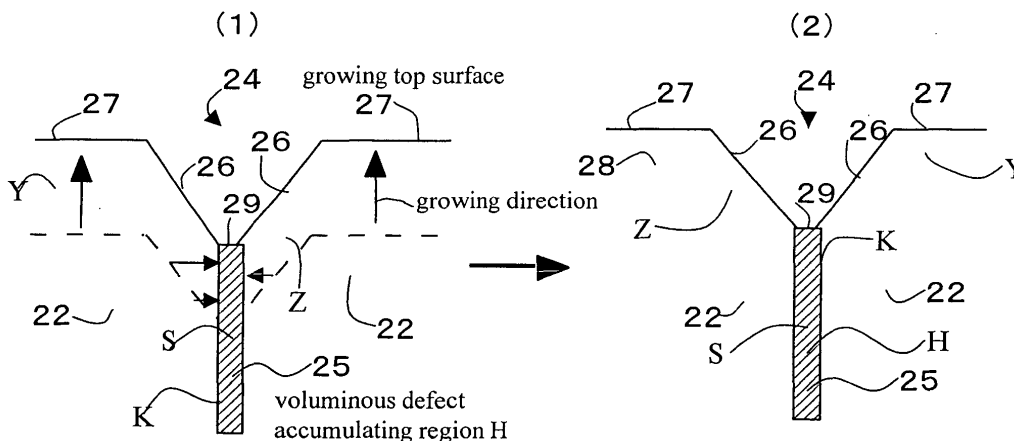
Fig.4 Growing method of the present invention
