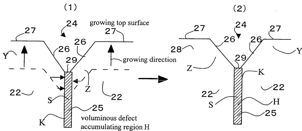
Fig.4 Growing method of the present invention
