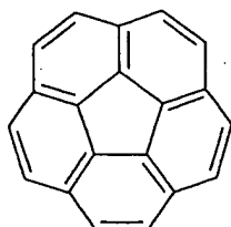
Coranurene
