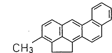
3-Methylcoranthracene
