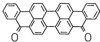
Violanthrone
