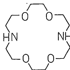
4,13-diaza-18-crown 6-ether
