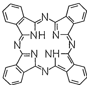
Phthalocyanine
