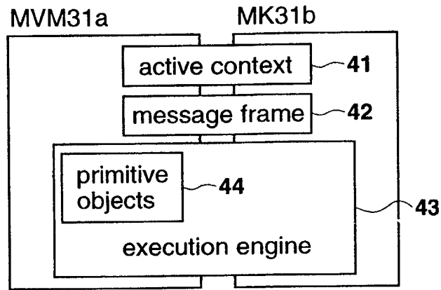
logical structure of MVM and MK
