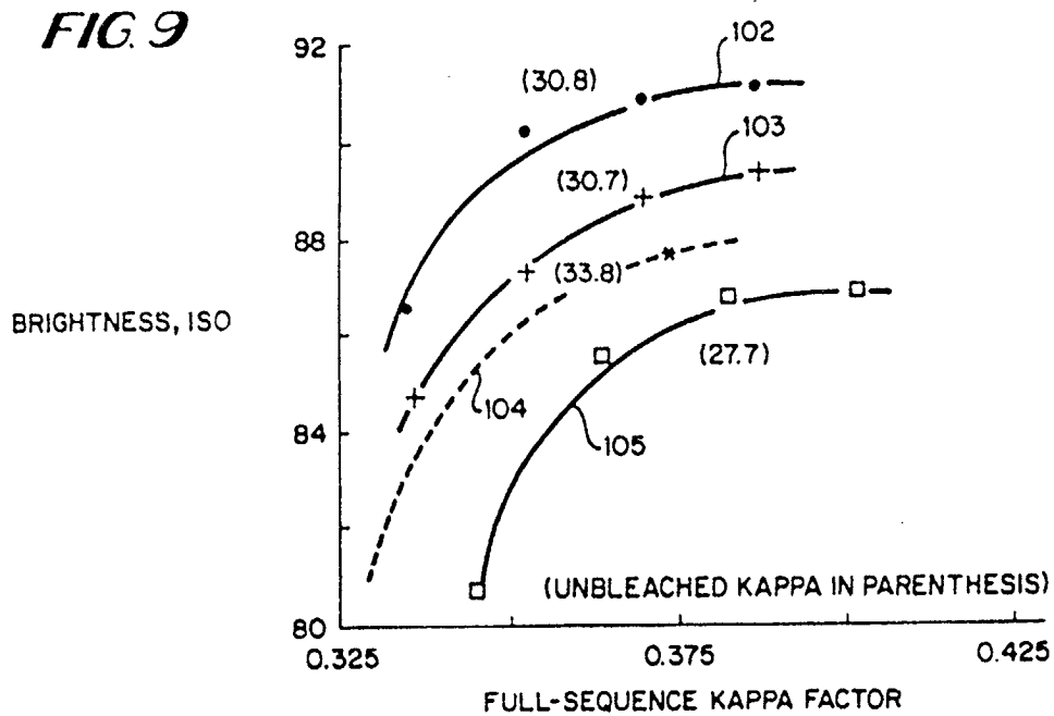
COMPARISON OF BRIGHTNESS RESPONSE FOR PULPS COOKED WITH DIFFERENT LIQUORS
