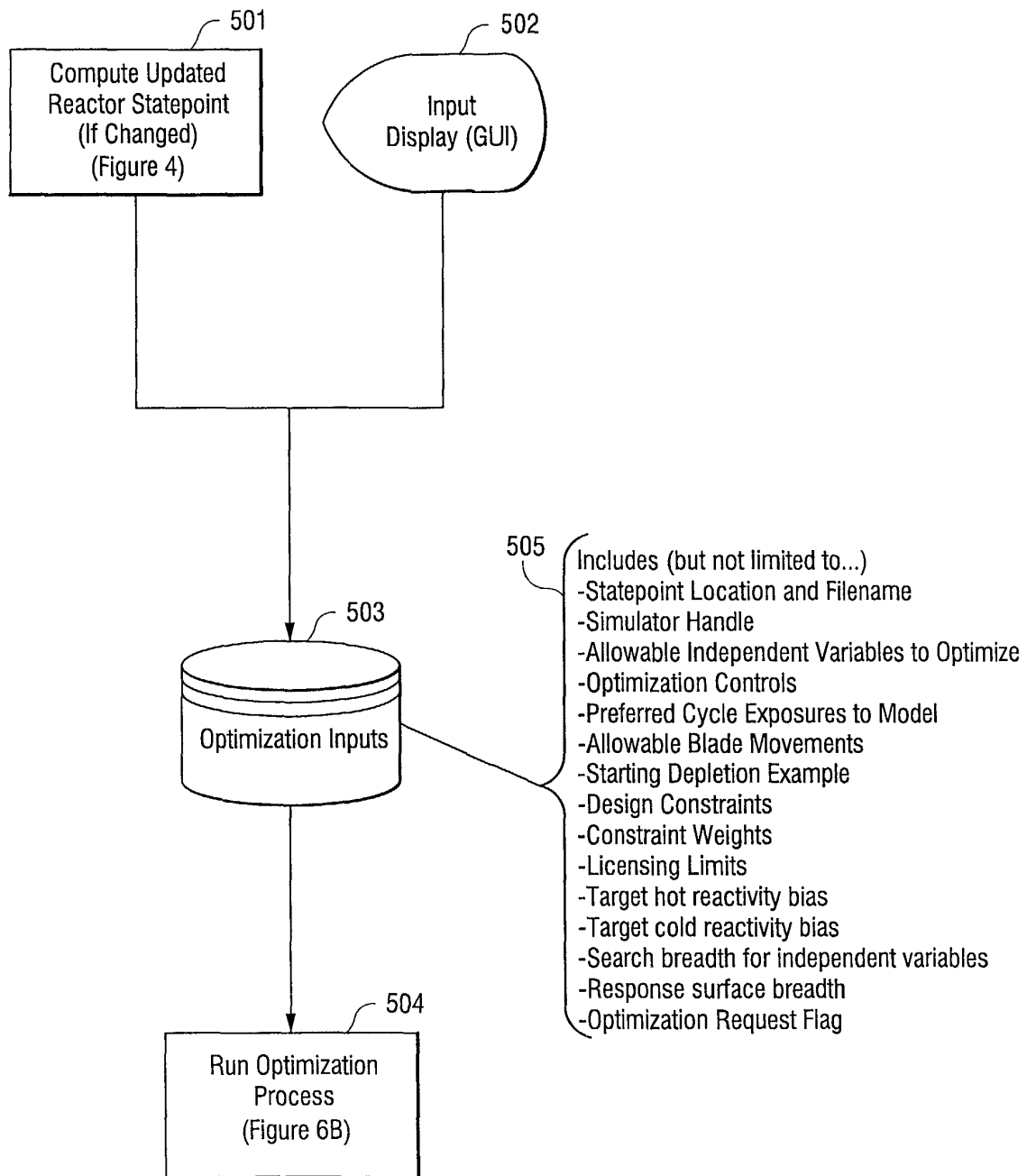
Fig. 5 Optimization Inputs Database
