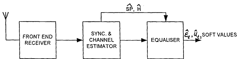
Fig. 2 PRIOR ART
