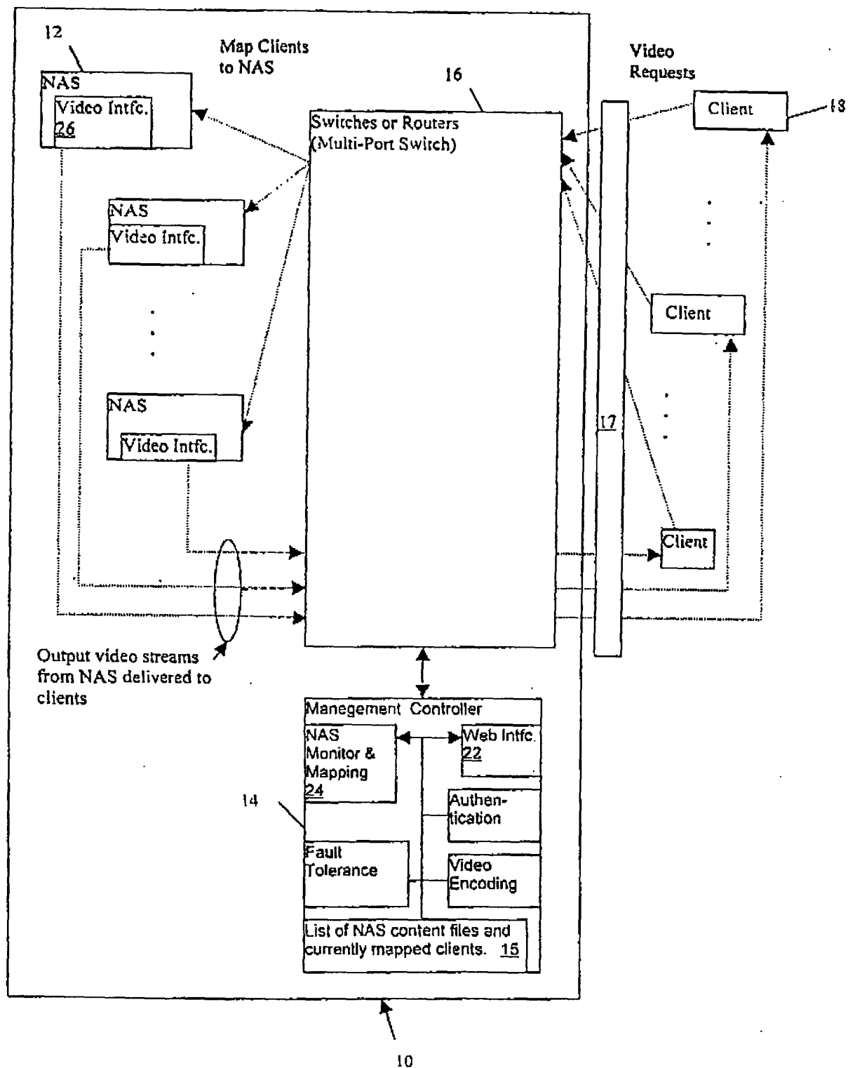
FIG. 2 - Video data flow with the distributed scalable video server
