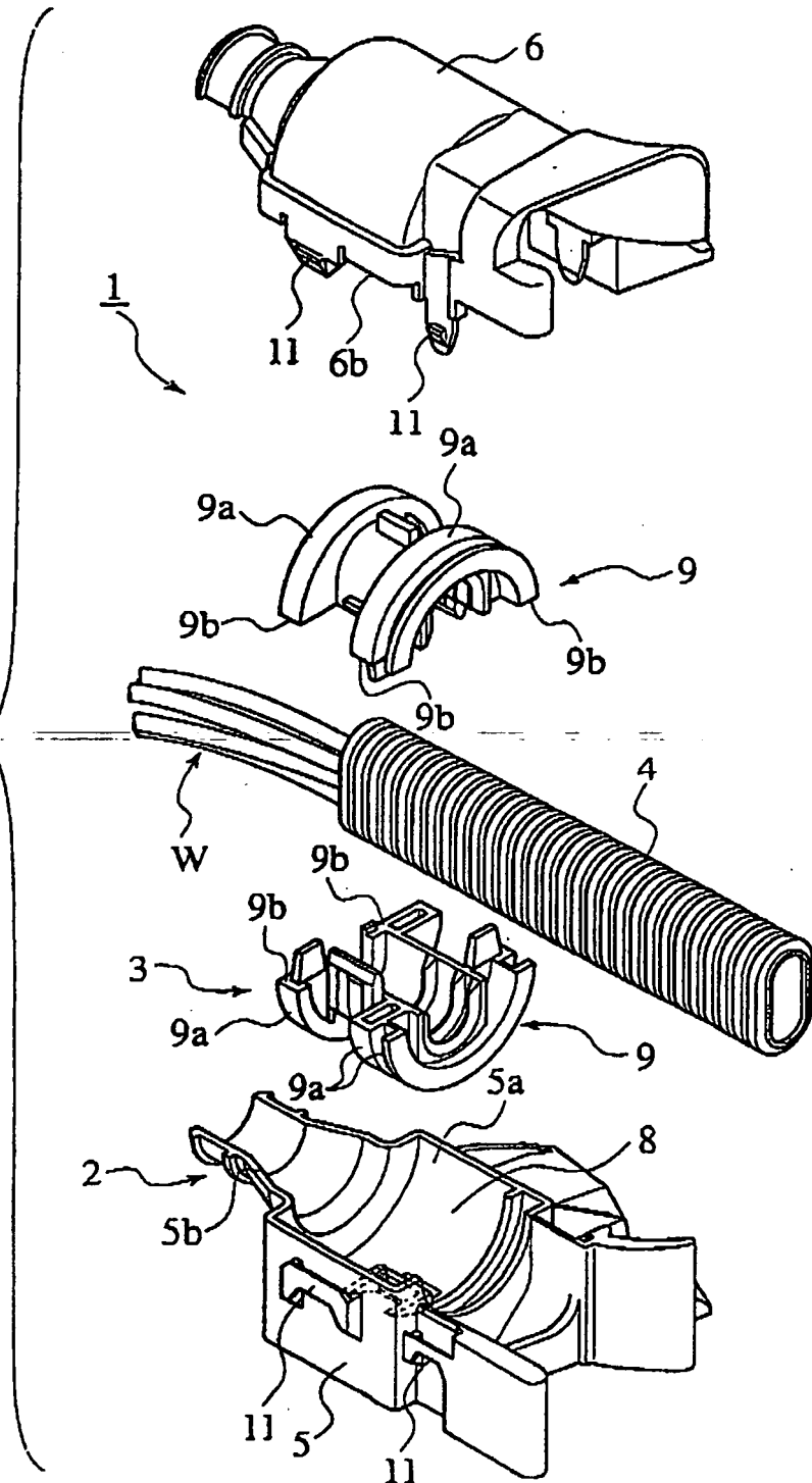
FIG. 1 PRIOR ART
