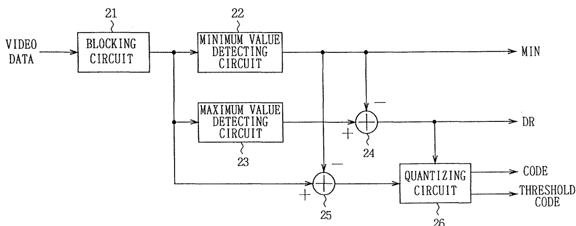
ADRC PROCESSING CIRCUIT
