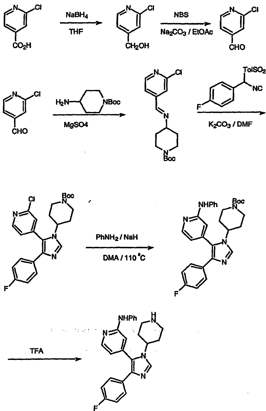
Scheme XI
