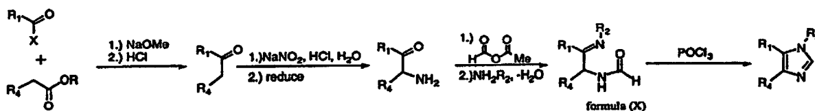
SCHEME II
