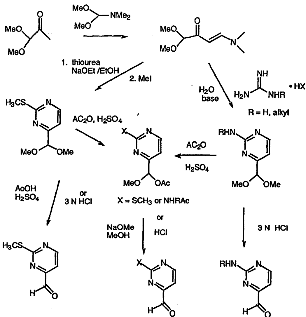
Scheme VIII
