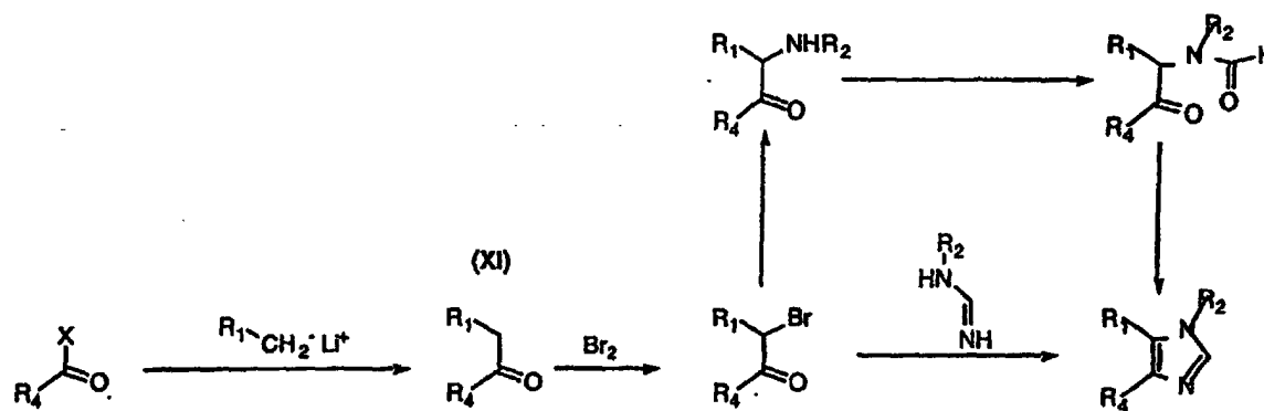
SCHEME III
