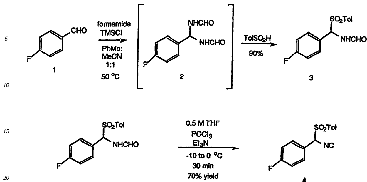
SCHEME XII
