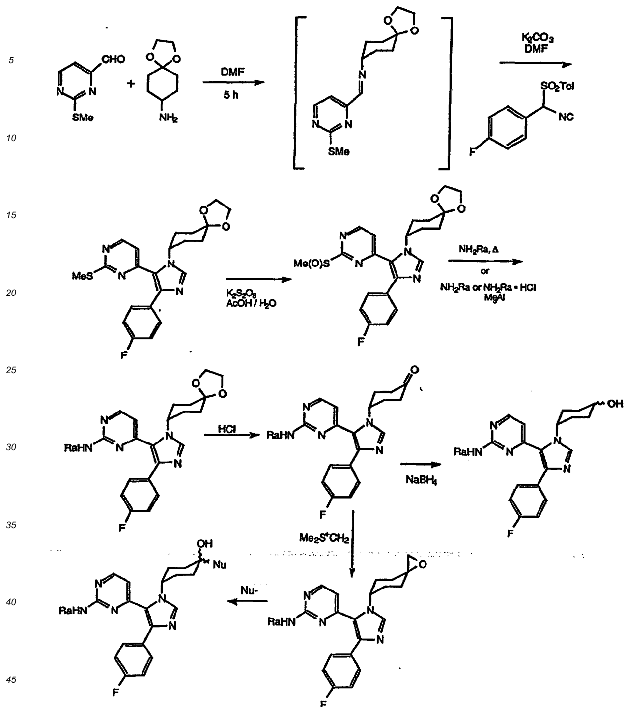
Scheme X
