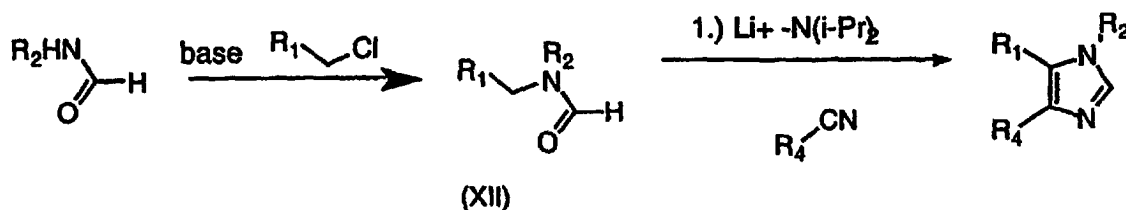
SCHEME IV
