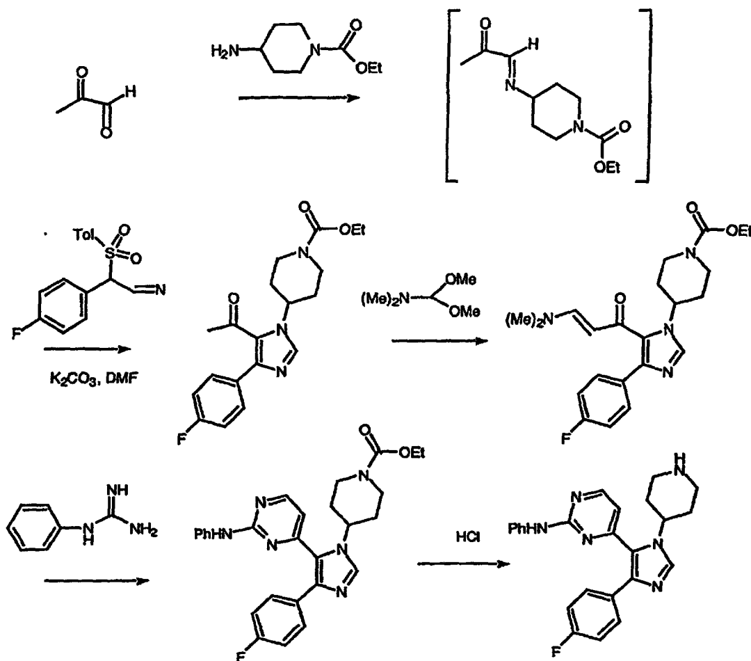
Scheme IX
