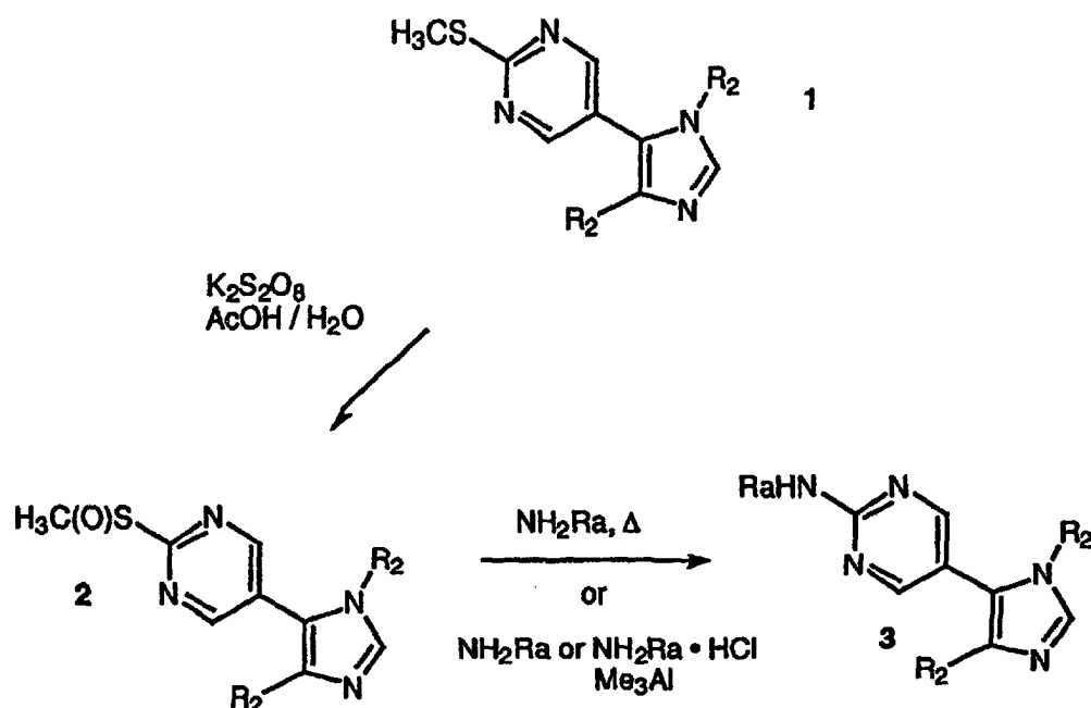
Scheme VII
