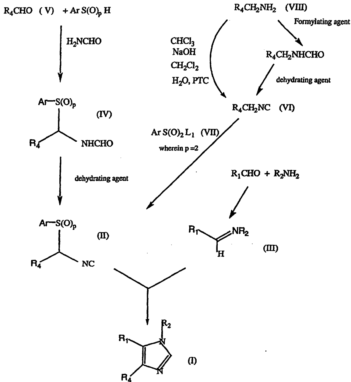
SCHEME I
