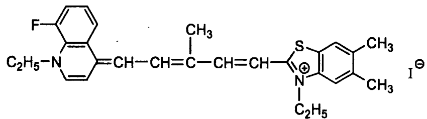
VIa-12
