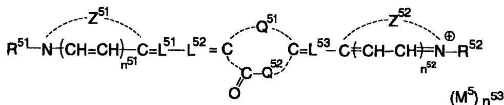
Formula (V)
