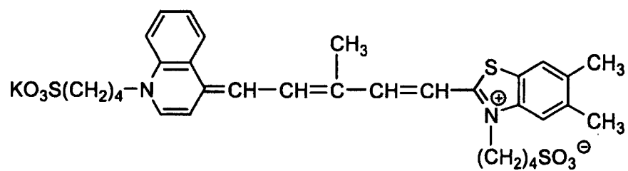
VIa-12
