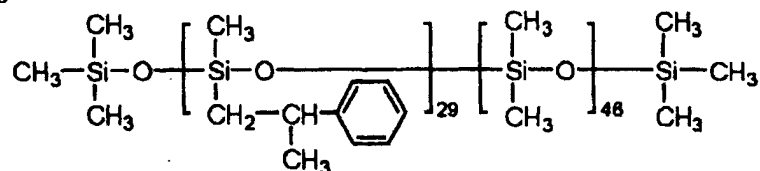
Cpd-10
