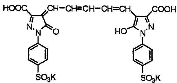
Cpd-18
