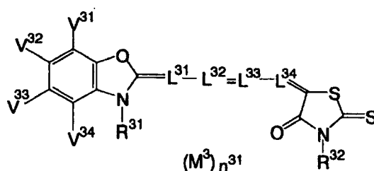
Formula (III)
