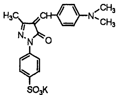
Cpd-15
