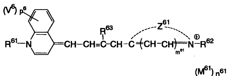
Formula (VIa)
