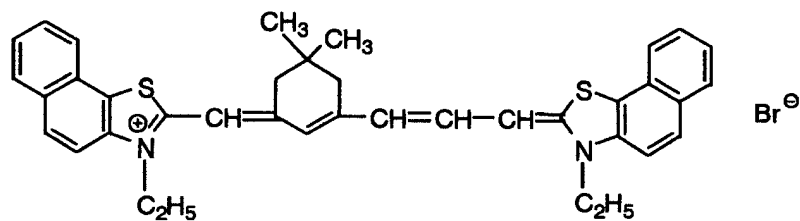
VIb-12
