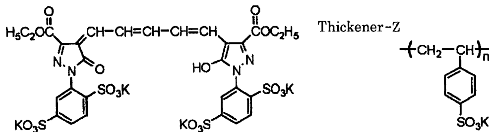
Cpd-14
