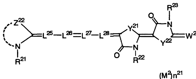
Formula (IIa)
