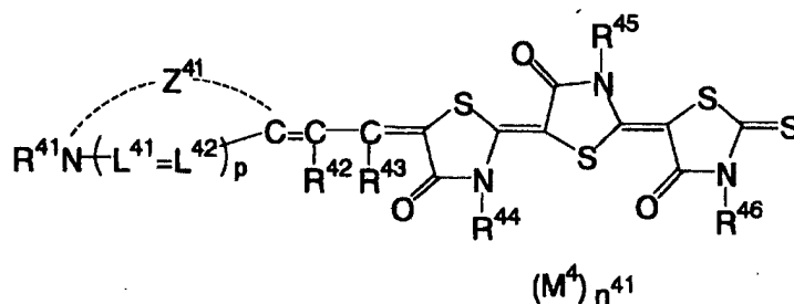
Formula (IV)
