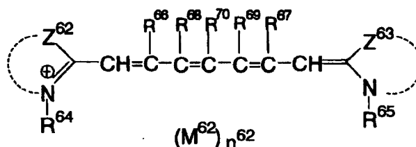
Formula (VIb)
