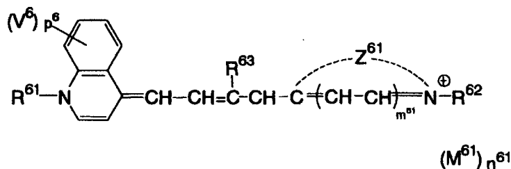
Formula (VIa)
