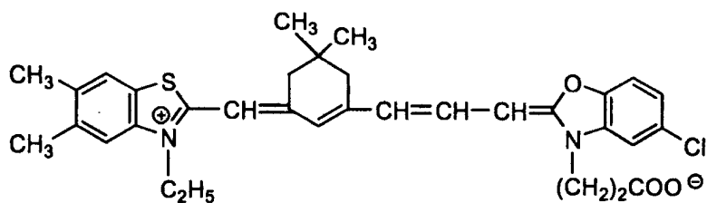
VIb-8
