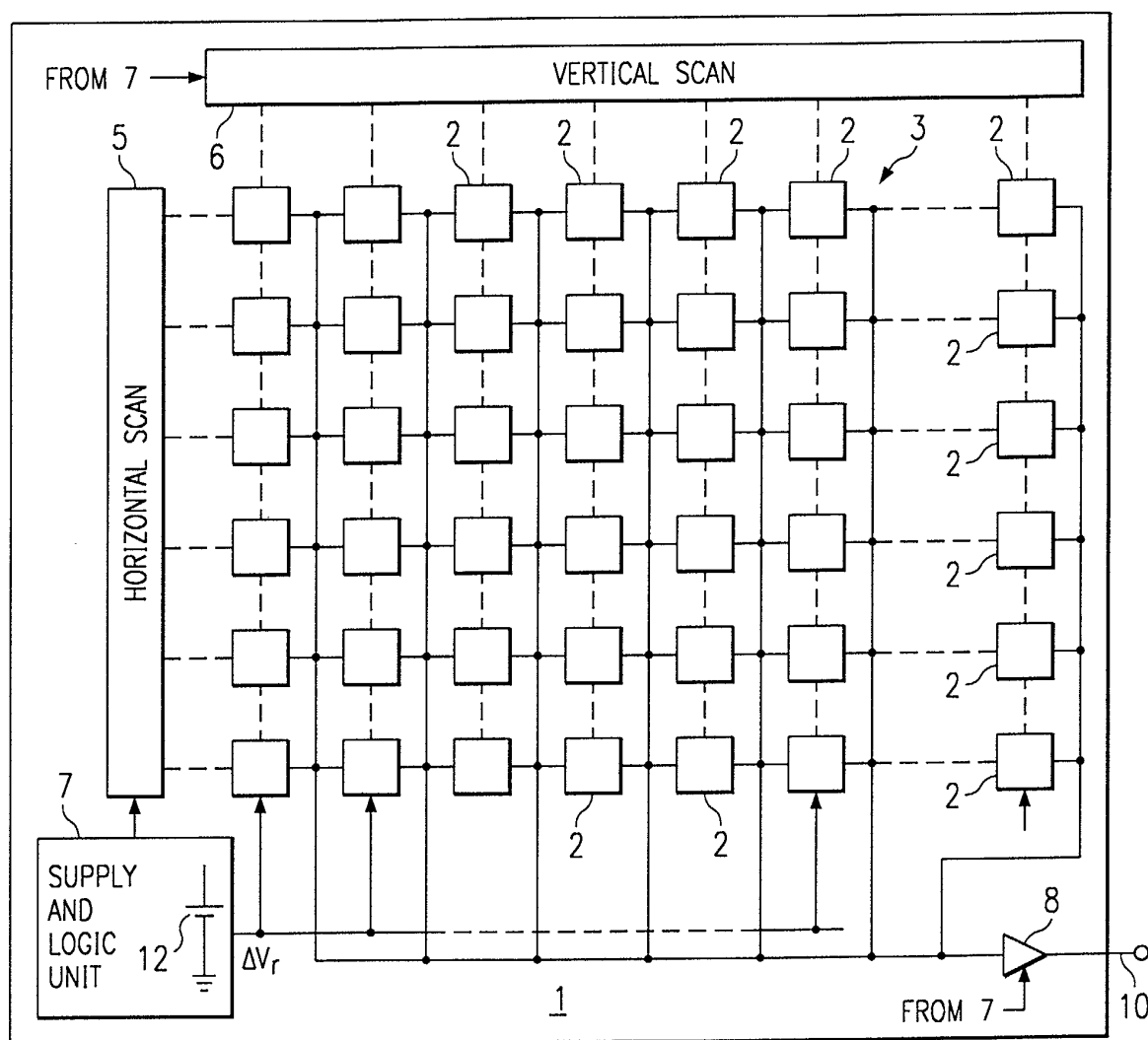
FIG. 1 (PRIOR ART)
