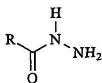
hydrazide
