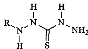
thiocarbazine
