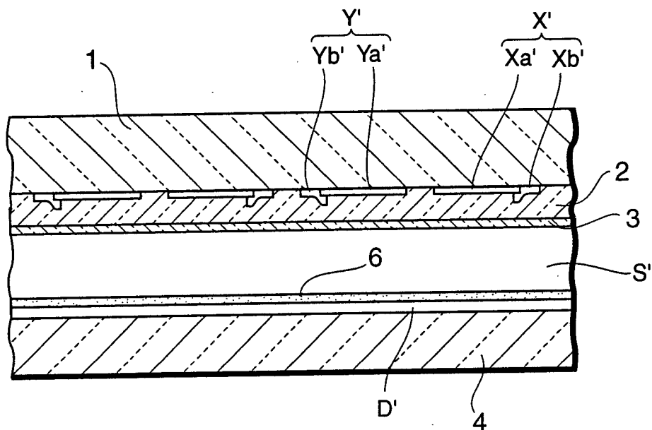
FIG.16 PRIOR ART W—W SECTION
