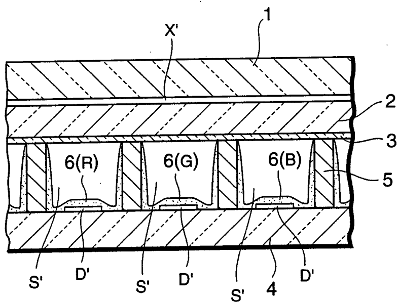
FIG.16 PRIOR ART W—W SECTION
