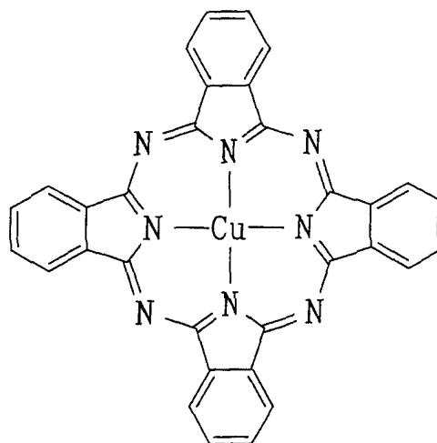
Copper(II) phthalocyanine(Cupc)
