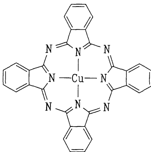
Copper(II) phthalocyanine(Cupc)
