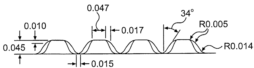
SIDE VIEW
