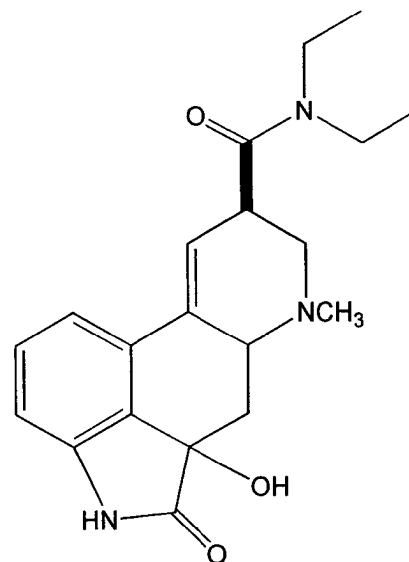
2-oxo-3-hydroxy-LSD 4
