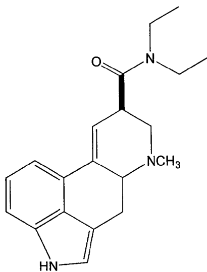
LSD 1
