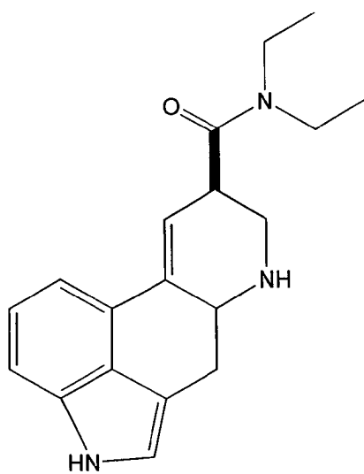
nor-LSD 3
