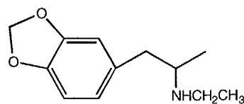
2 MDEA (Eve)
