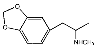
1 MDMA (Ecstasy)
