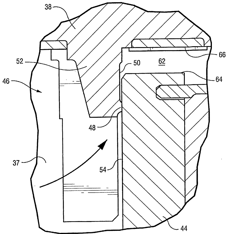
Fig. 2 (Prior Art)
