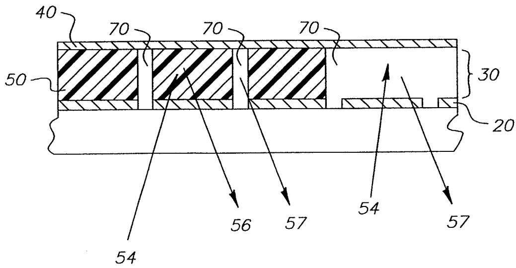
FIG. 7A (PRIOR ART)
