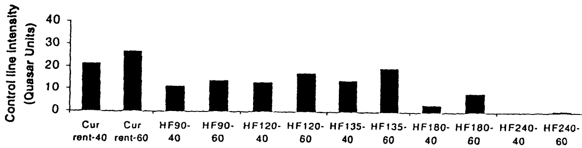
Figure 2 - Comparison of control line signal at 40 and 60 sec for nitrocellulose of different flow rates using 400 mIU/mL hCG urine standard
