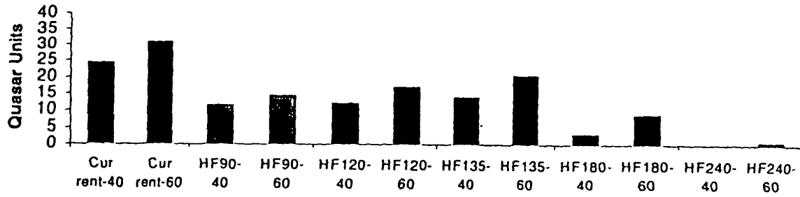
Figure 1 - Comparison of control line signal at 40 and 60 sec for nitrocellulose of different flow rates using 0 mIU/mL hCG urine standard
