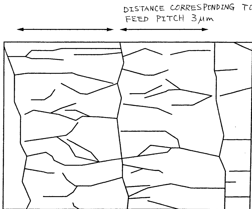
FIG.11B ILLUSTRATIONS SHOWING CRYSTAL GRAIN BOUNDARY OF FIG.11A
