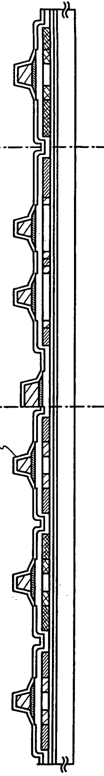
FIG. 8C FORMATION OF FIRST INTERLAYER INSULATING FILM/LASER ACTIVATION
