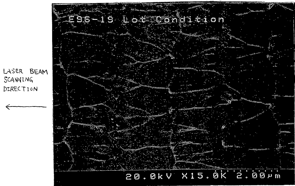
FIG.11A SEM OBSERVATION AFTER LASER CRYSTALLIZATION (X15K) (CRYSTAL GRAIN BOUNDARY IS VISUALIZED IN A MANNER OF SECCO ETCHING)
