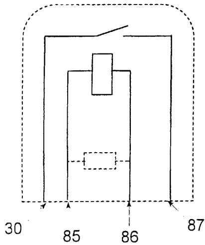
FIG 14 (PRIOR ART)
