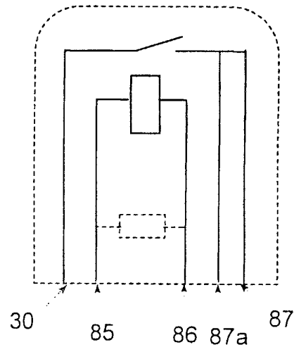
FIG 15 (PRIOR ART)
