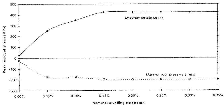
Figure 3: Effect of levelling extension on maximum residual stress level (residual stress near the mid-thickness position).
