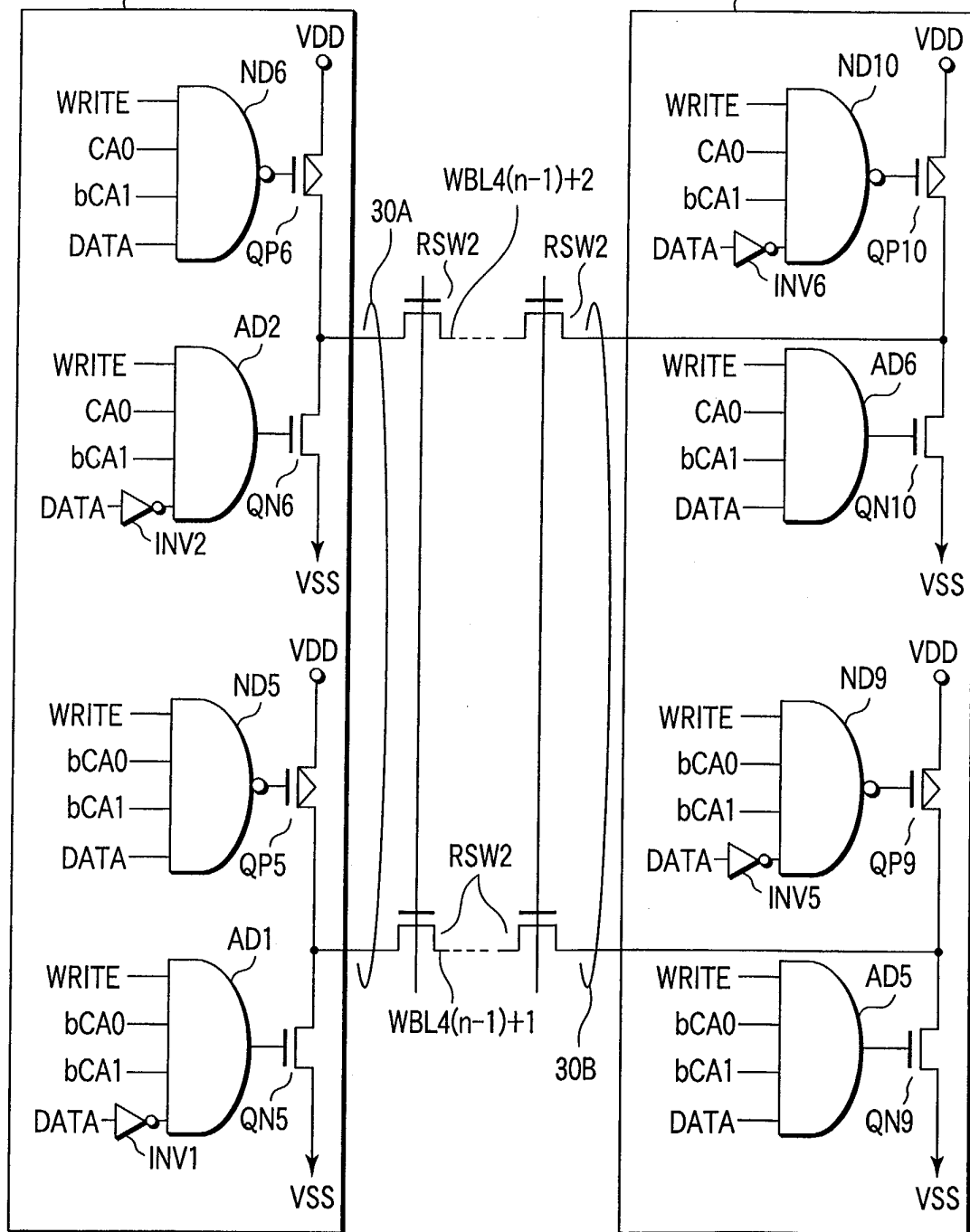
Write bit line driver/sinker 23AS
