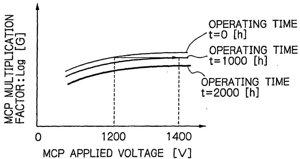
CORRELATION BETWEEN MCP APPLIED VOLTAGE AND MCP MULTIPLICATION FACTOR
