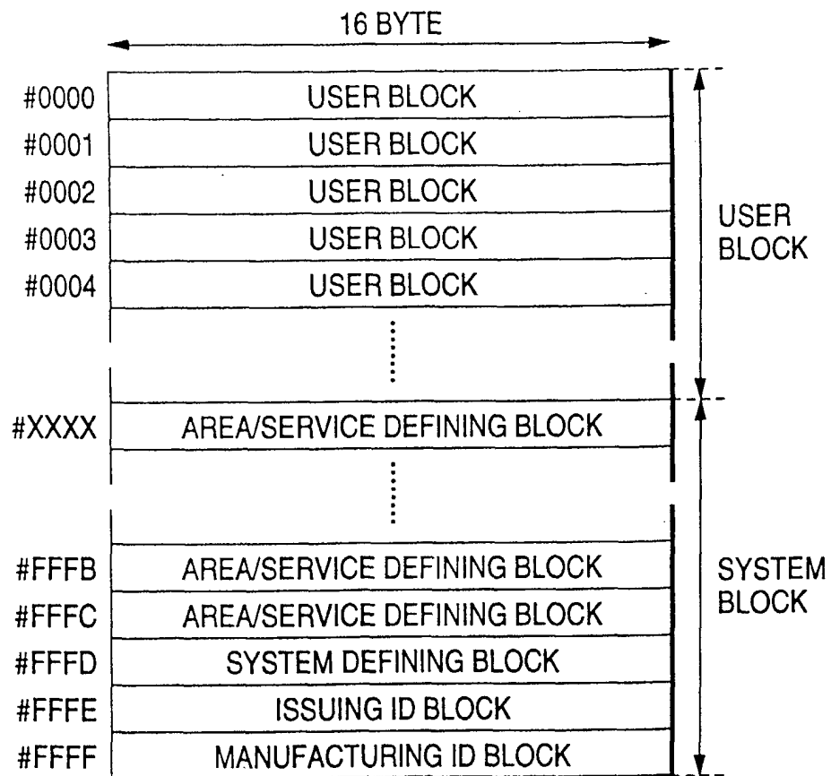
LOGICAL FORMAT OF EEPROM 66
