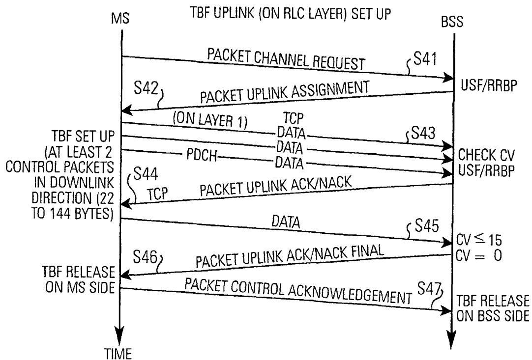
FIG.4 PRIOR ART
