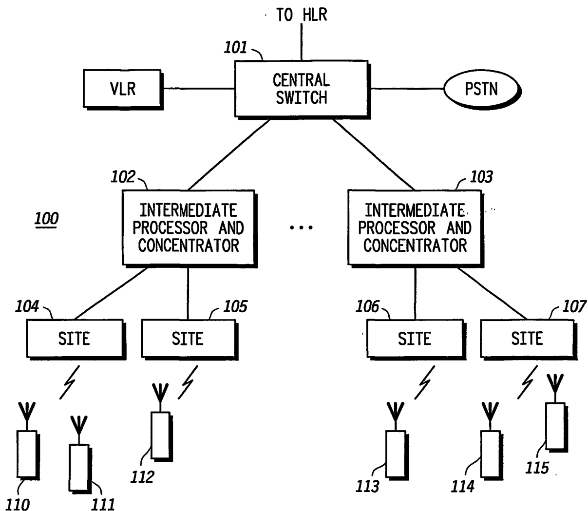
FIG.1 -PRIOR ART-
