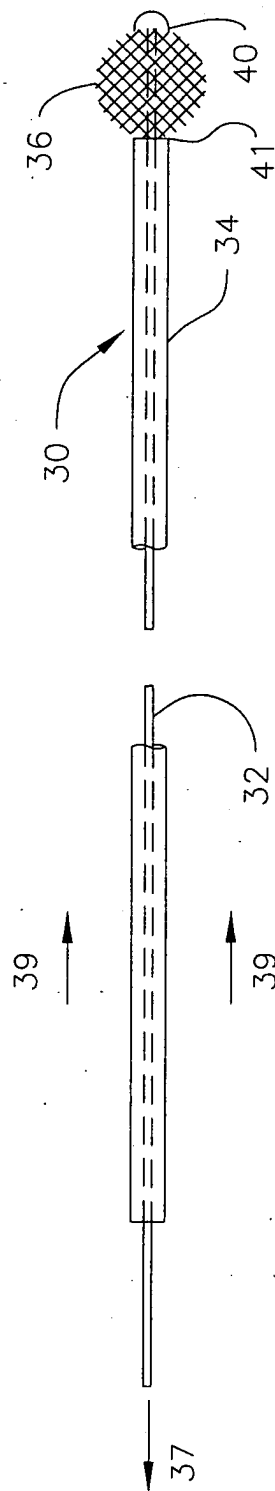
FIG. 4 (PRIOR ART)
