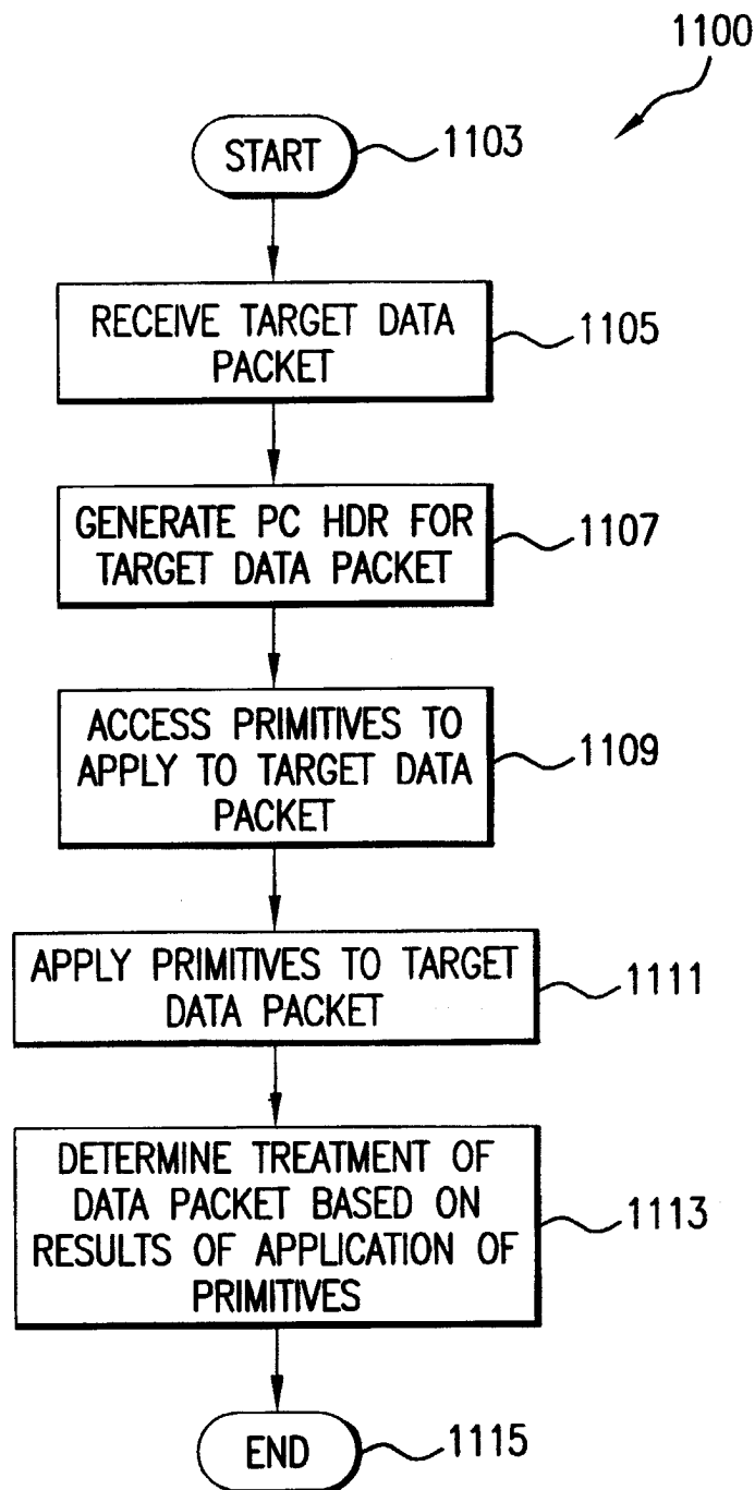
FIG.11 TEST APPLICATION
