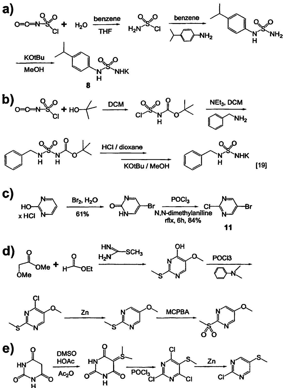
Scheme 3: Preparation of the sulfamide-moieties [10], [11], [12], [13], [14], [15] and [19] and preparation of substituted pyrimidines [16], [17]:
