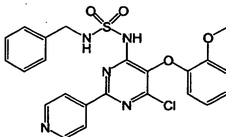
LC-MS: t_R : 4.68; [M+H]^+ : 498.14
