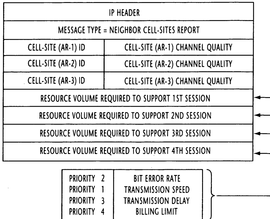
FIG. 10 CANDIDATE NOTIFICATION MESSAGE (ICMP)
