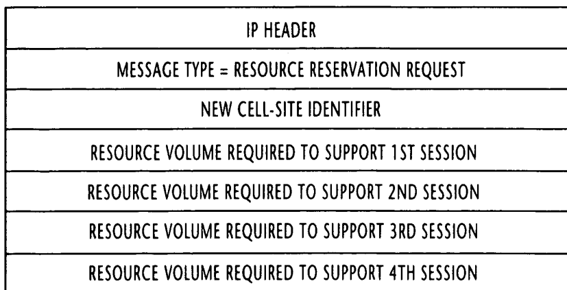
FIG. 11 RESOURCE RESERVATION REQUEST MESSAGE-1 (ICMP)
