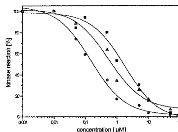
Figure 1: Dose-response curves of CDK1/cyclin B kinase inhibition by 3-isopropyl-5-methyl-7-benzylamino-pyrazolo[4,3-d]pyrimidine (●), 3-isopropyl-5-chloro-7-benzylamino-pyrazolo[4,3-d]pyrimidine (▲), 3-isopropyl-5-(4-hydroxycyclohexylamino)-7-benzylamino-pyrazolo[4,3-d]pyrimidine (■).
