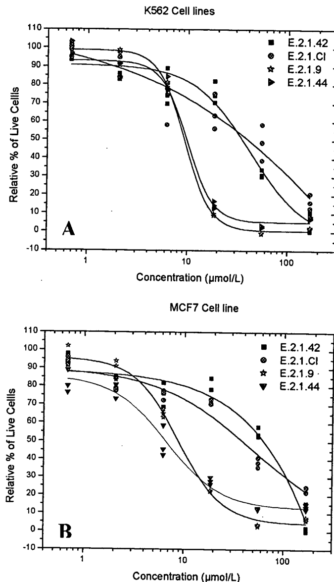
Figure 6: Inhibition of growth of K562 (A) and MCF7 (B) tumour cell lines by different pyrazolo[4,3-d]pyrimidines. Cytotoxicity was determined in the presence of Calceim AM. Activity is presented as percentage of maximal activity (in the absence of inhibitors). E.2.1.Cl: 5-chloro-7-benzylamino-3-isopropylpyrazolo[4,3-d]pyrimidine; E.2.1.9: 269 - 5-( R )-(1-hydroxymethylpropyl)amino-7-benzylamino-3-isopropylpyrazolo[4,3-d]pyrimidine; E.2.1.42: 268 - 5-(4-aminocyclohexyl)amino-7-benzylamino-3-isopropylpyrazolo[4,3-d]pyrimidine; E.2.1.44: 5-(4-hydroxycyclohexyl)amino-7-benzylamino-3-isopropylpyrazolo[4,3-d]pyrimidine.
