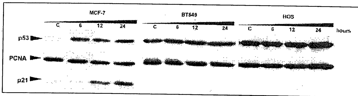
Figure 16: Effect of 25 on p53 and p21 WAF1 induction in cells expressing either wild-type or mutant p53 protein. Total cell lysates were separated on 12,5% SDS gel. Immunoblotting was performed with monoclonal anti-p53 antibody DO-1, anti-p21 antibody 118 and subsequently with anti-PCNA antibody PC-10, to confirm equal protein loading. Panel A shows, that 20 \mu M 25 is able to induce p53 protein as well as p21 WAF1 protein in MCF-7 cells expressing wild-type p53. On the contrary, panels B and C show, that 20 \mu M 25 failed to induce these proteins in BT549 and HOS cells expressing mutant p53 protein.
