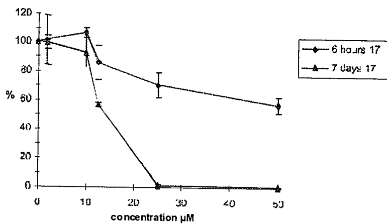
Figure 4: a. Growth curve CEM + 1, b. Growth curve CEM + 172, c. Growth curve CEM + 47
