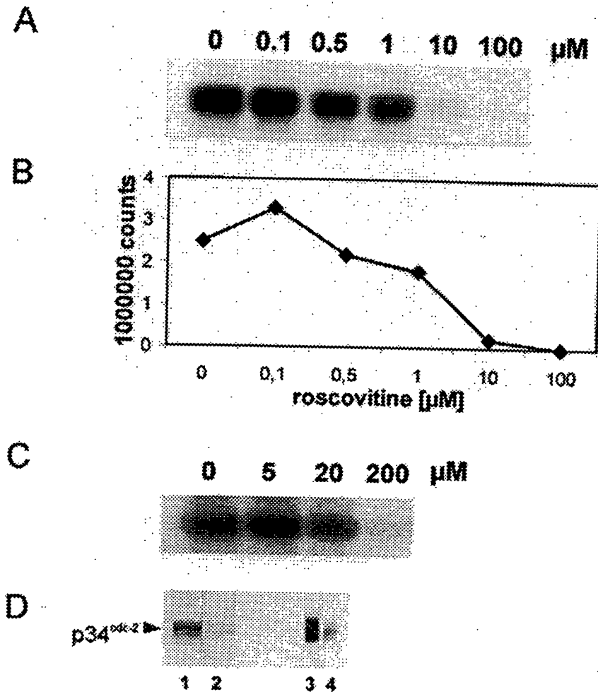
Figure 2: Specific inhibition of cdc2Ms kinase activity by 3-isopropyl-5-(4-aminocyclohexylamino)-7-benzylamino-pyrazolo[4,3-d]pyrimidine ( 268 ) in cells of V. faba . Enzyme activity measured by phosphorylation of histone H1 substrate protein in presence of various concentration of roscovitine. (A) Phosphoimmager (B) Inhibition of cdc2Ms kinase in vivo in cells treated with various concentrations of roscovitine (D). Total cdk protein level as detected by Western blots of whole cell extracts. Control (lane 1), 48h of treatment with 268 (lane 2). W. Blot of suc 1 bound cdks – control (line 3), 48h of 268 treatment
