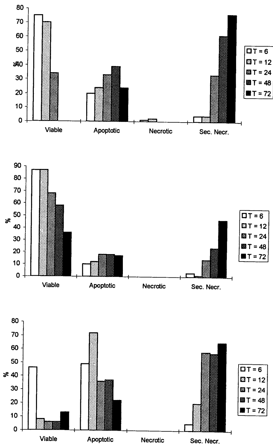
Figure 12: Microscopic detection of viable, apoptotic, necrotic and secondary necrotic cells in CEM cultures incubated with a.98 b.172 c.201 (T: time of incubation with compounds in hours).
