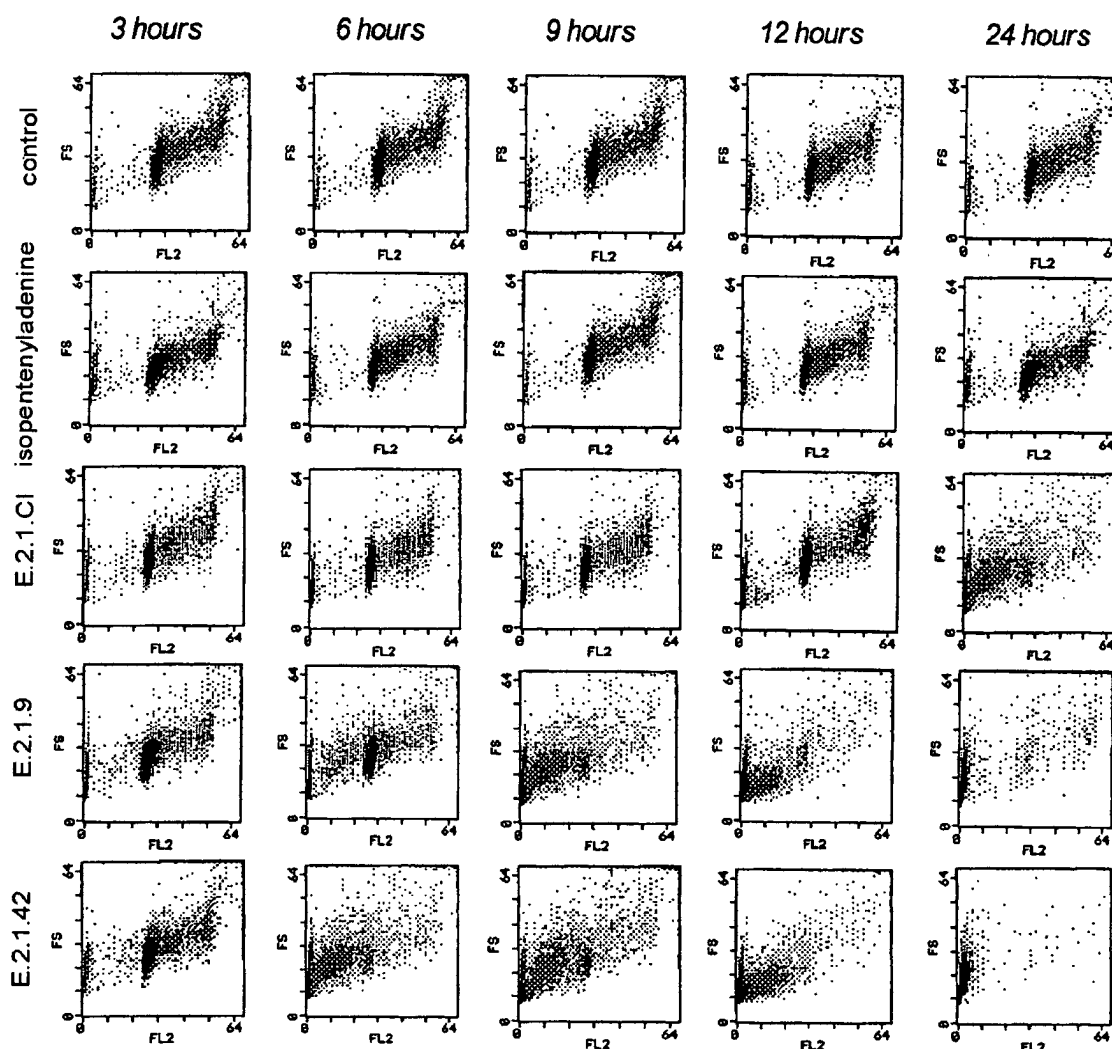
Figure 14: Synthetic CDKIs induce apoptosis in CEM cells – FACS study.
