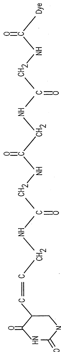
Tetraglycinyllinker
