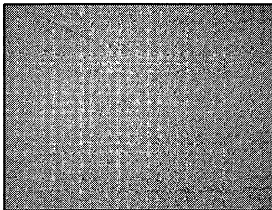
Fig. 6c MIN. SPANGLE GALVALUME - 0.04% Ti, 0.008% B
