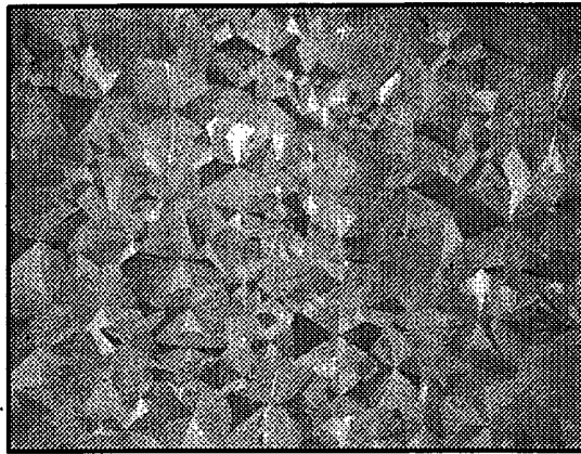
Fig. 6a NORMAL GALVALUME - NO \text{TiB}_2 ADDITION
