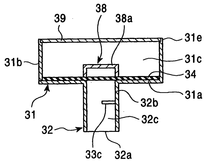
FIG. 11 PRIOR ART
