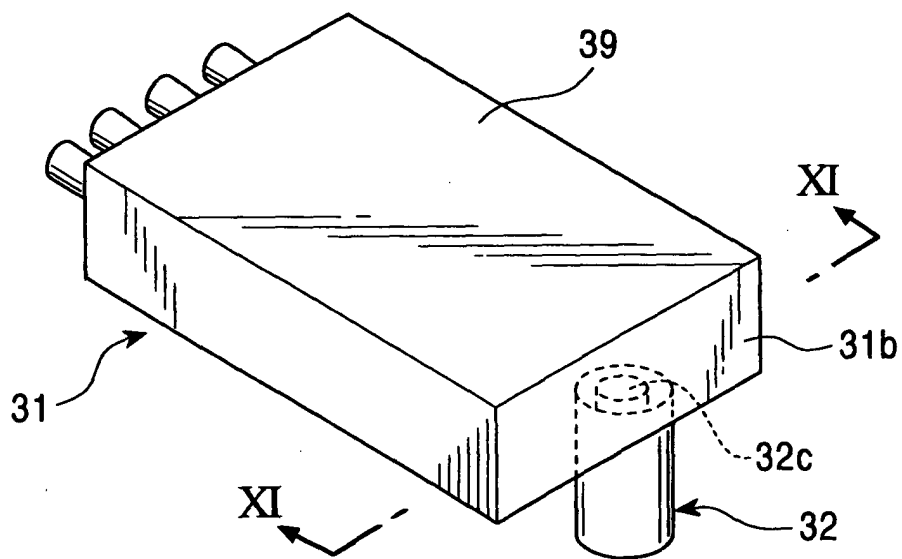
FIG. 10 PRIOR ART
