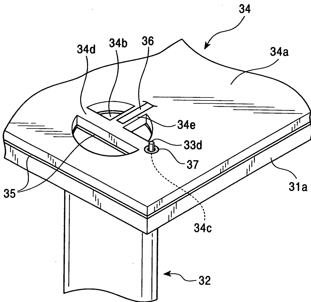
FIG. 13 PRIOR ART
