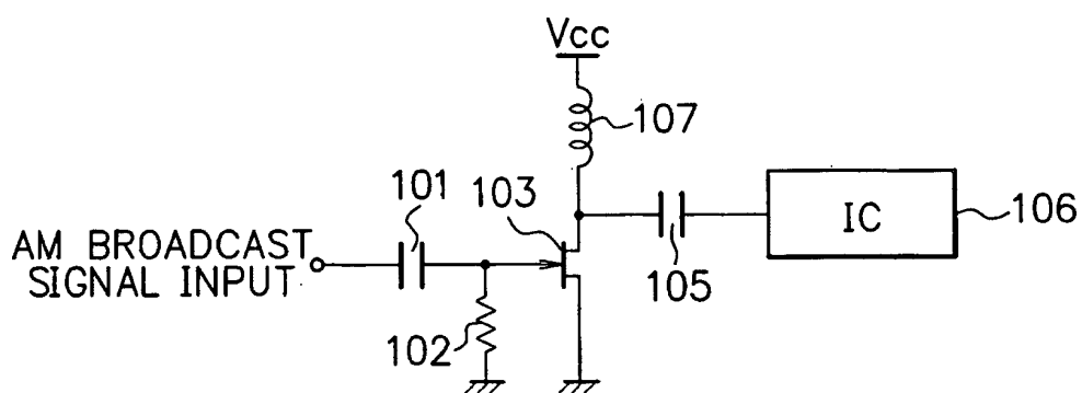
(b) NON-TUNING CIRCUIT FORMAT
